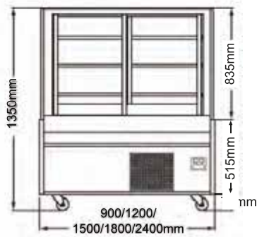
Back View
